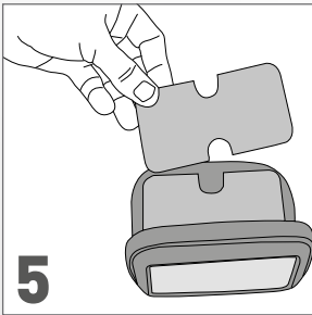
5 Insert the shims provided with the unit until the suitably shimmed navigator touches the clear surface of the case
